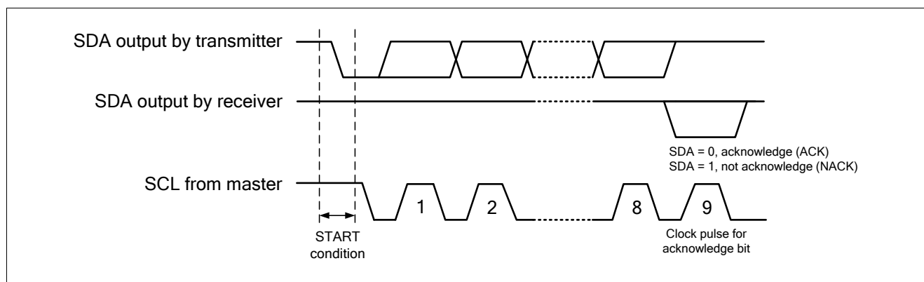
Figure 15.5. Acknowledge Bit
