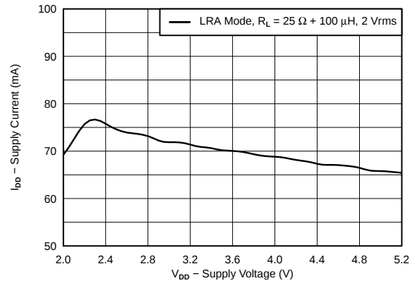
Figure 10. Supply Current vs Supply Voltage (Full Vibration)
